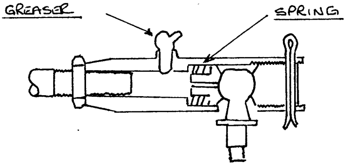
TRACK ROD ENDS
