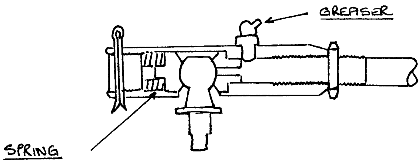
STEERING DROP ARM JOINTS BEARING CUP EITHER SIDE OF BALL
