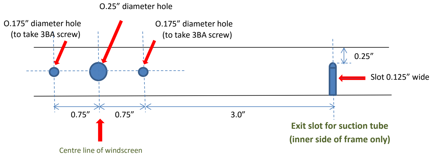
Wiper motor mounting holes (through both sides of frame)
